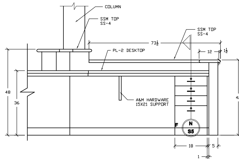
18 9 REFERENCE DESK 101 ARCHITECTURAL REF: 1/A4-002/OPP. SCALE: 3/8" = 1'
