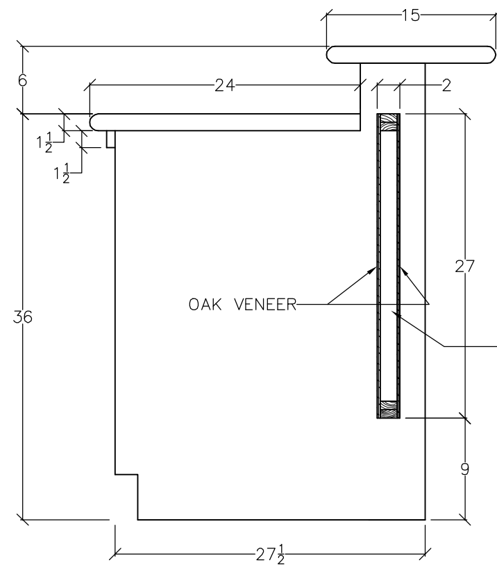
GATE @ CIRC. DESK SCALE: 1" = 1'
