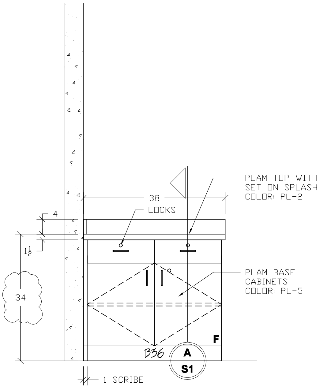
COPY ROOM 136 ARCHITECTURAL REF: 4/A4-004 SCALE: 3/4" = 1'
