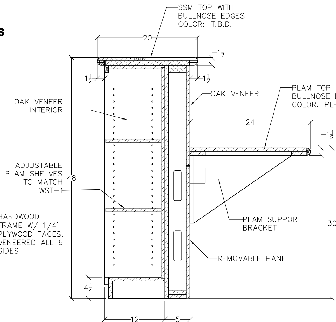
TEEN COUNTER DETAIL SCALE: 1" = 1'
