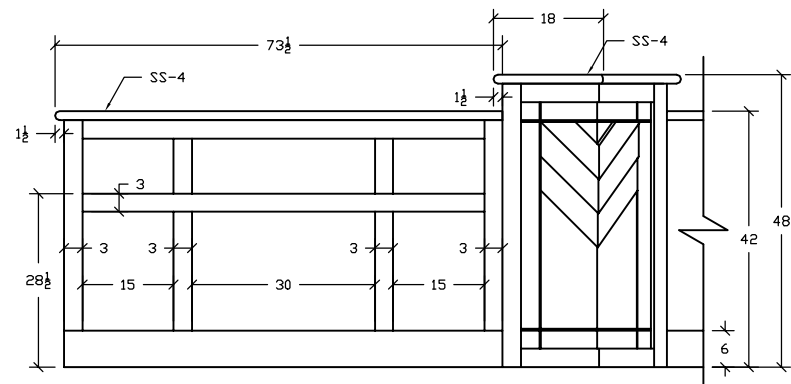
19 10 REFERENCE DESK 101 ARCHITECTURAL REF: 4/A4-002 SCALE: 3/8" = 1'
