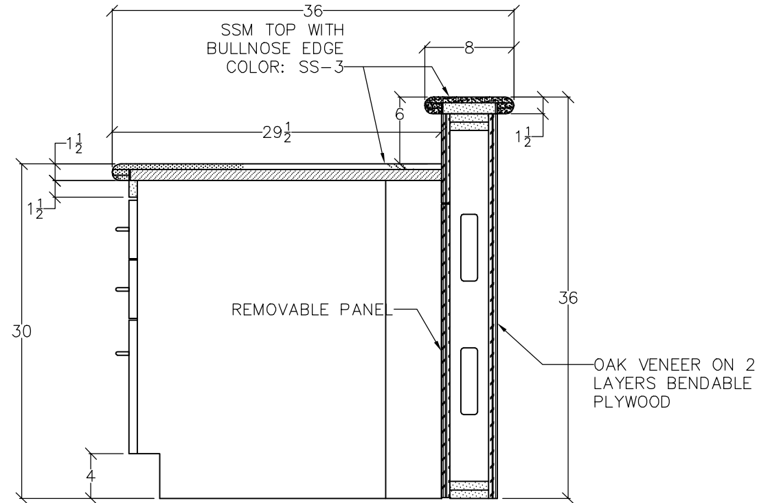
CC YOUTH COMPUTER DESK SCALE: 1" = 1'
