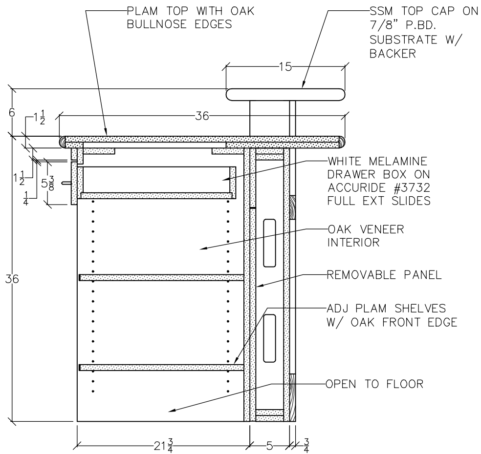
K CIRCULATION DESK SCALE: 1" = 1'
