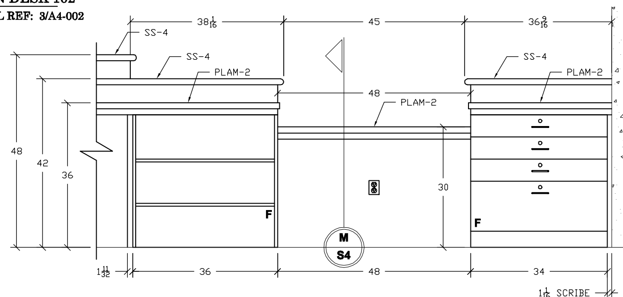
5 5 CIRCULATION DESK 102 ARCHITECTURAL REF: 5/A4-002 SCALE: 1/2" = 1'
