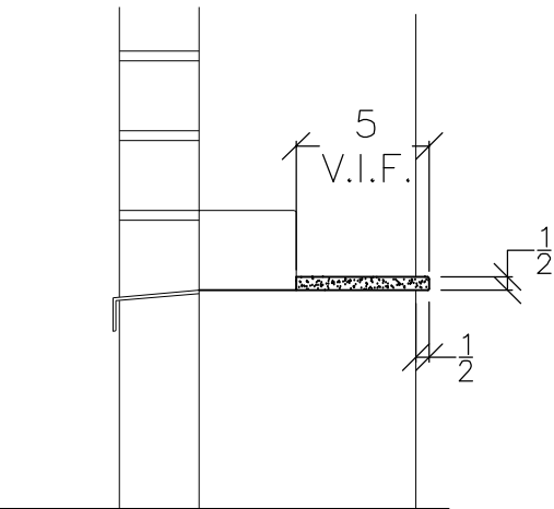
SILL DETAIL SCALE: 1-1/2" = 1' GVWP TO PROVIDE 315 FT
