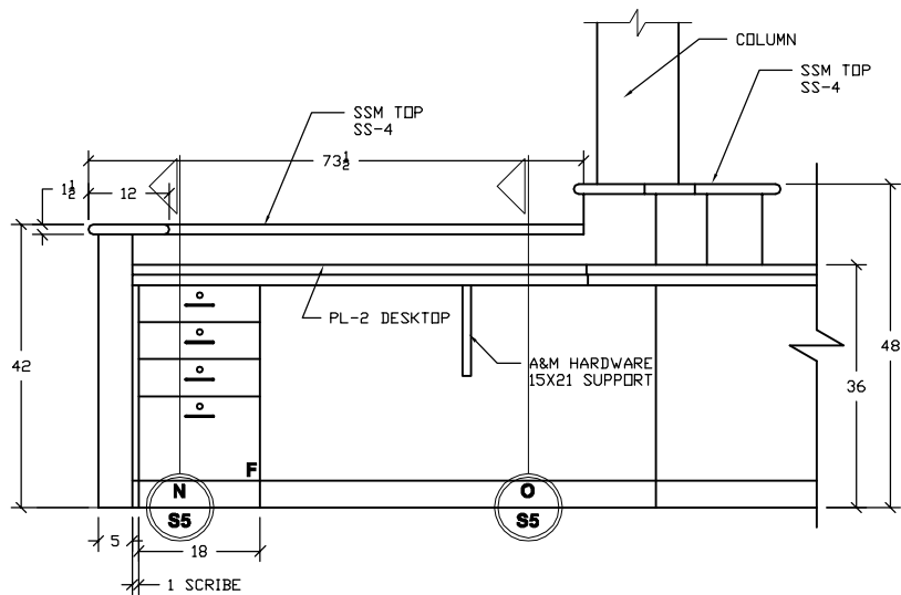
14 9 REFERENCE DESK 101 ARCHITECTURAL REF: 1/A4-002 SCALE: 3/8" = 1'
