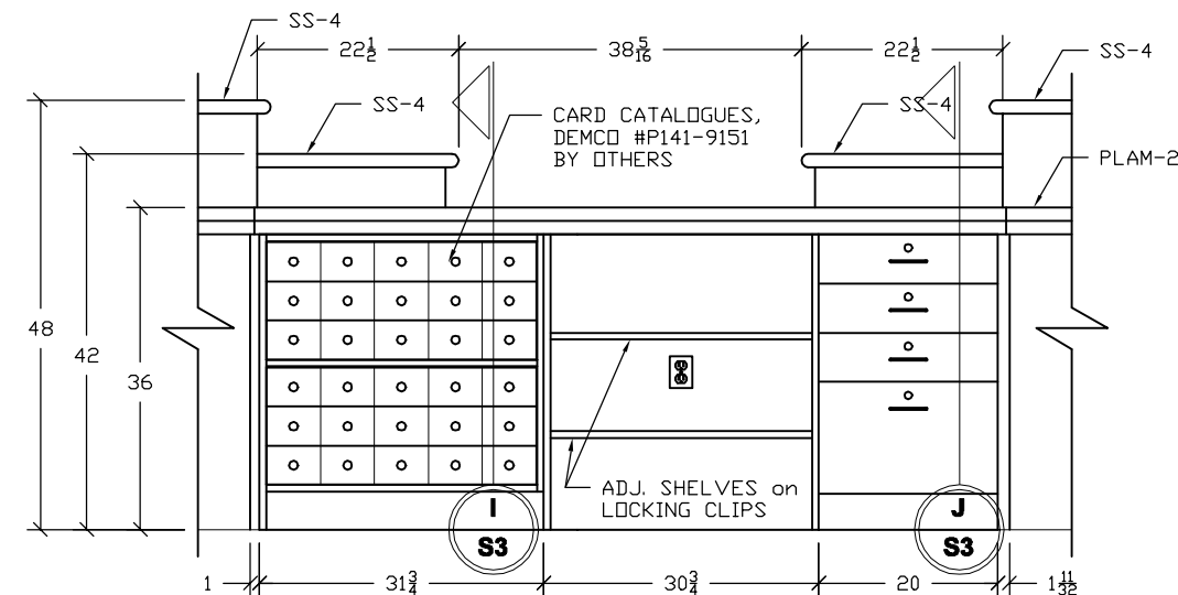
2 5 CIRCULATION DESK 102 ARCHITECTURAL REF: 2/A4-002 SCALE: 1/2" = 1'
