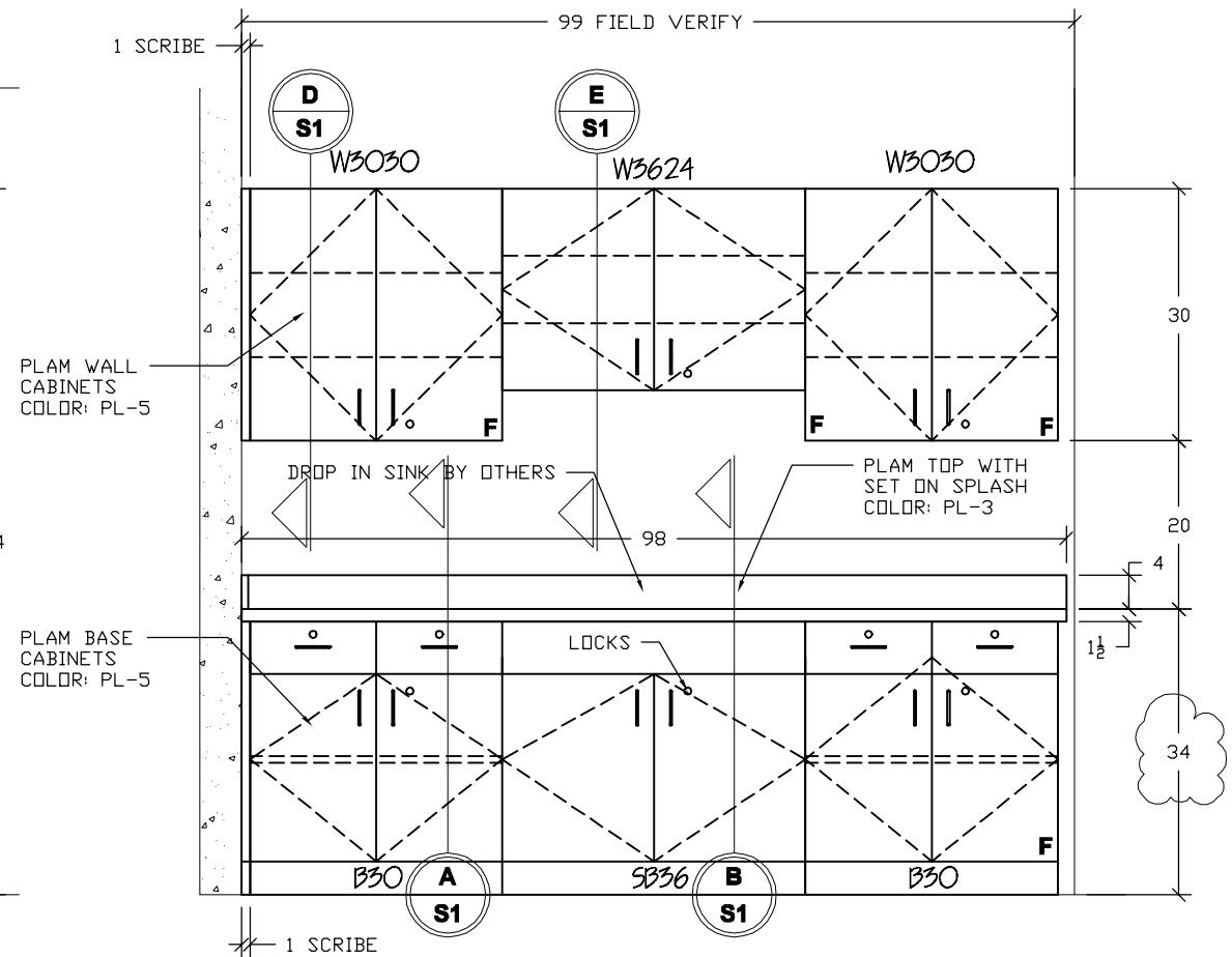
YOUTH PROGRAM ROOM 116 ARCHITECTURAL REF: 3/A4-005 SCALE: 1/2" = 1'
