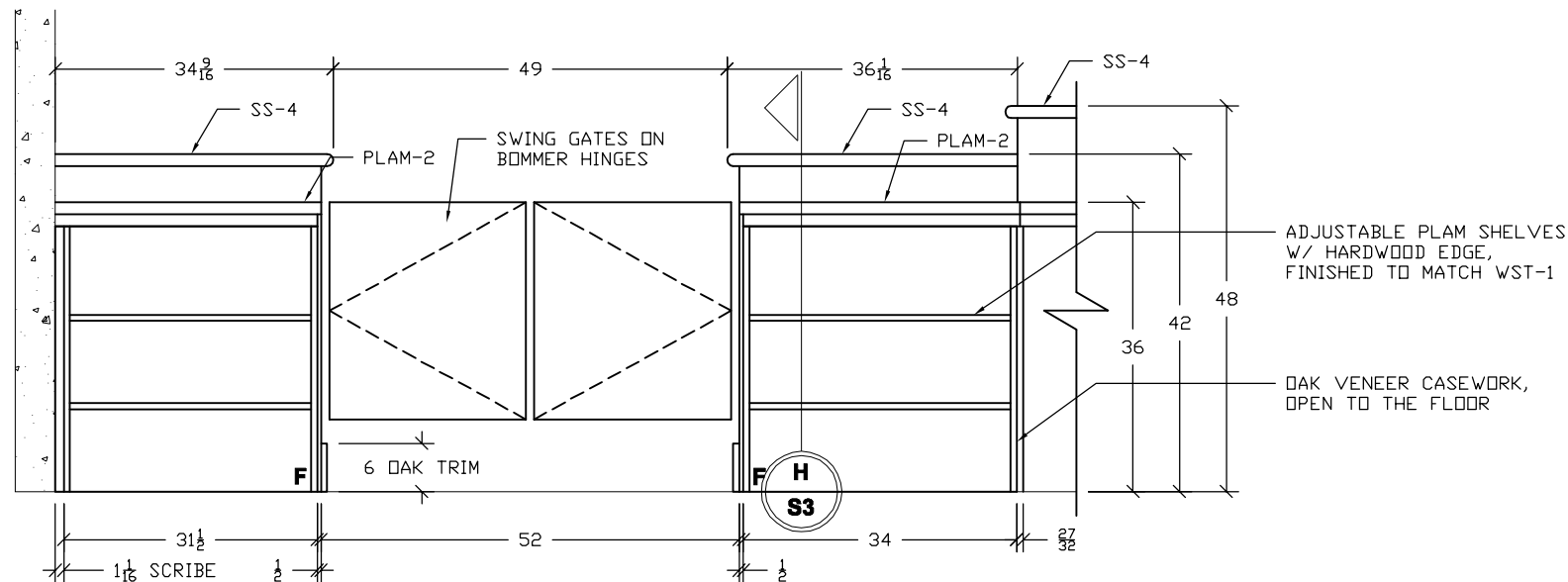
1 5 CIRCULATION DESK 102 ARCHITECTURAL REF: 1/A4-002 SCALE: 1/2" = 1'
