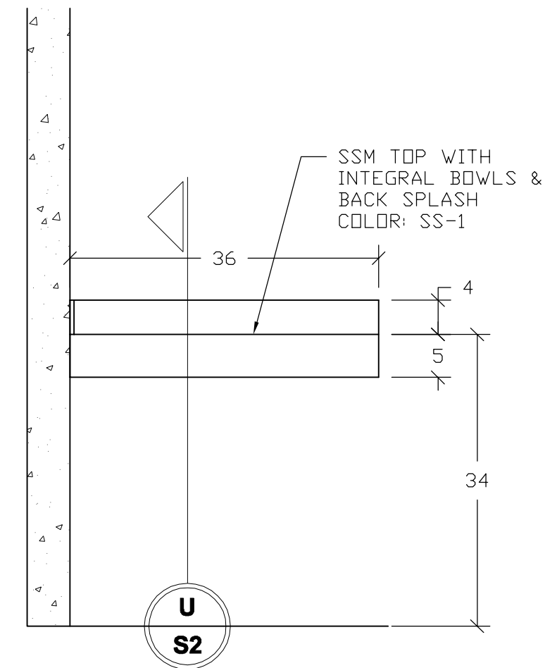
RESTROOM 104 ARCHITECTURAL REF: 3/A4-001 SCALE: 3/4" = 1'
