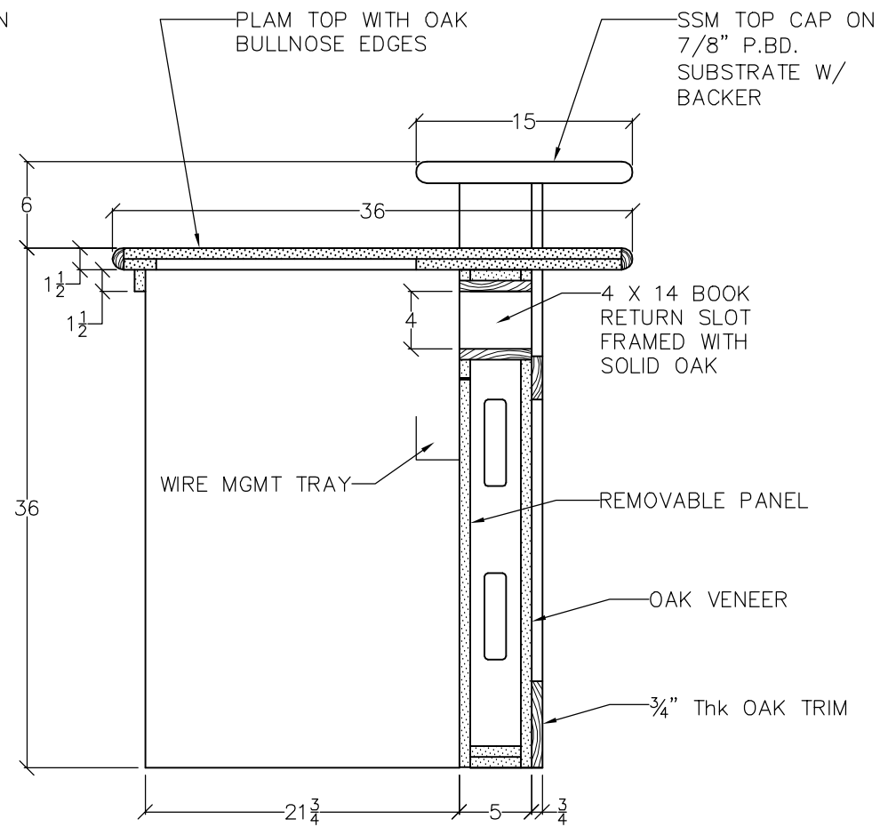
L CIRCULATION DESK SCALE: 1" = 1'
