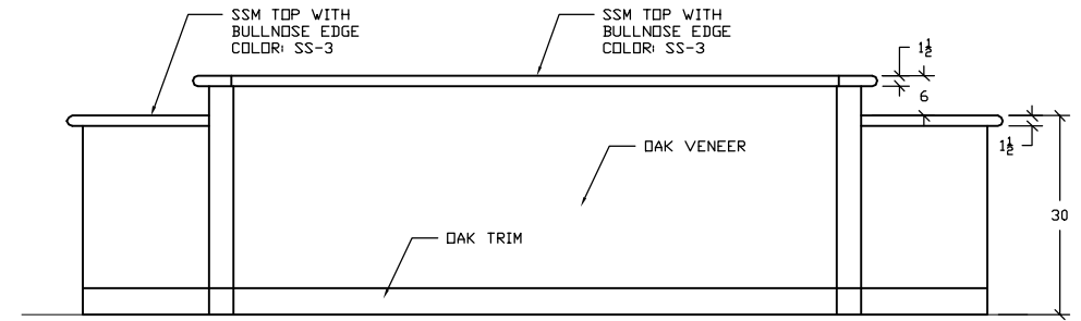
26 19 YOUTH COMPUTER DESK ARCHITECTURAL REF: 5/A4-006 SCALE: 3/8" = 1'
