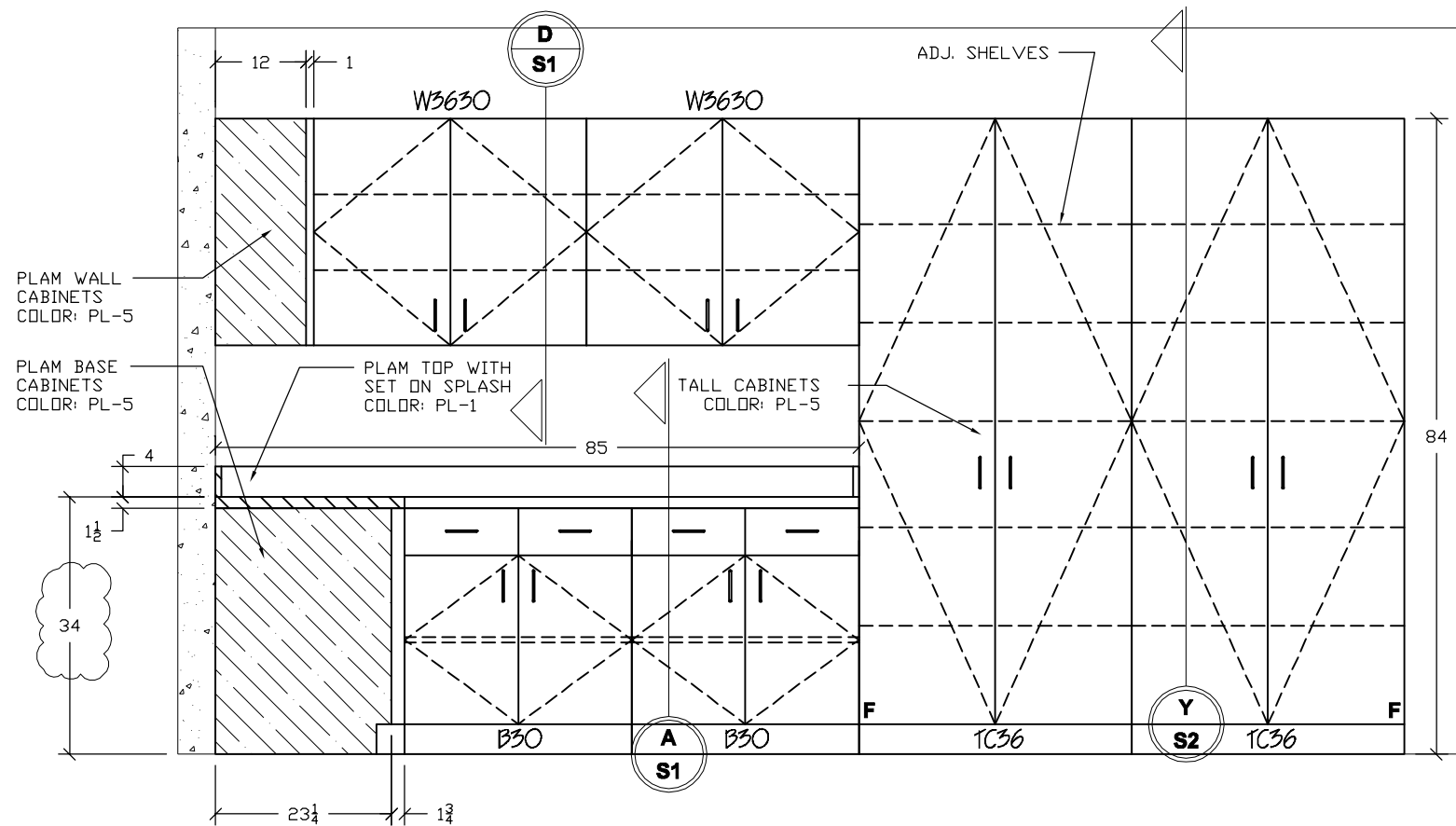
28 15A WORK ROOM 117 ARCHITECTURAL REF: 3/A4-005 SCALE: 1/2" = 1'
