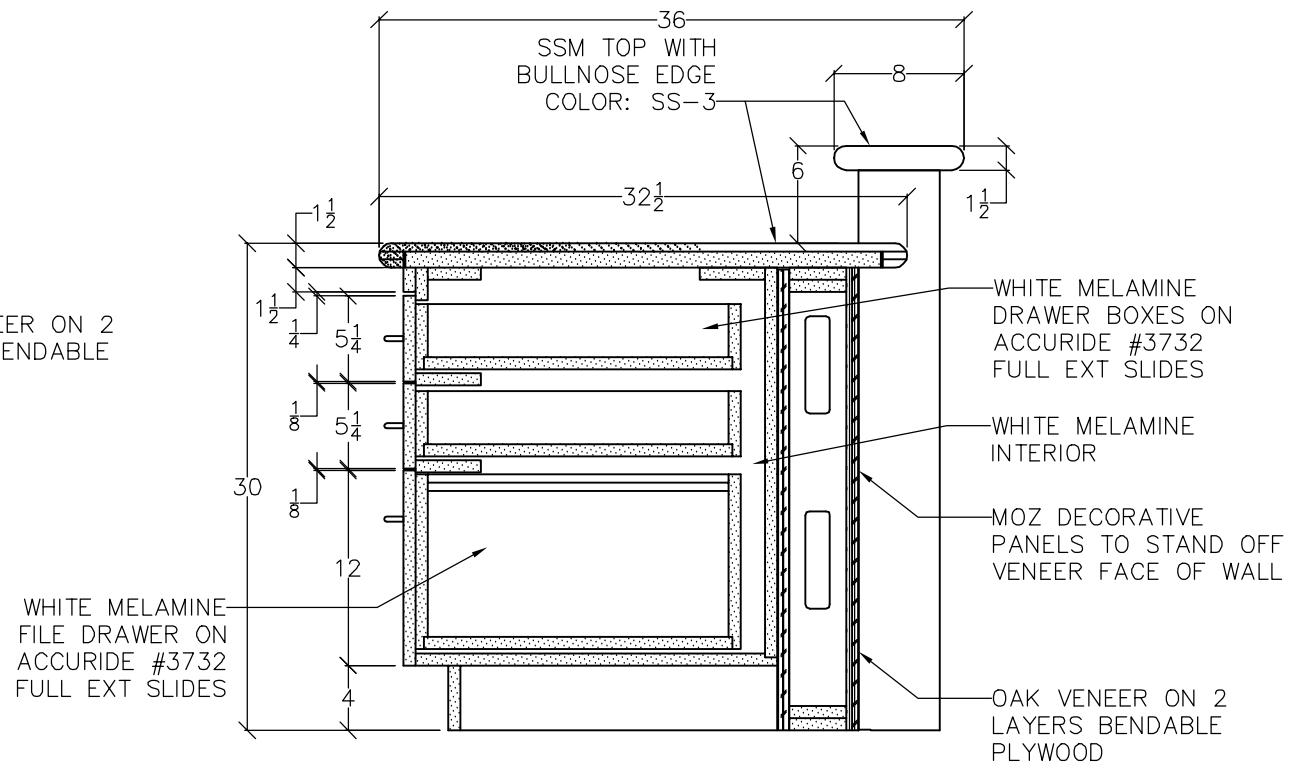
DD YOUTH REFERENCE DESK SCALE: 1" = 1'
