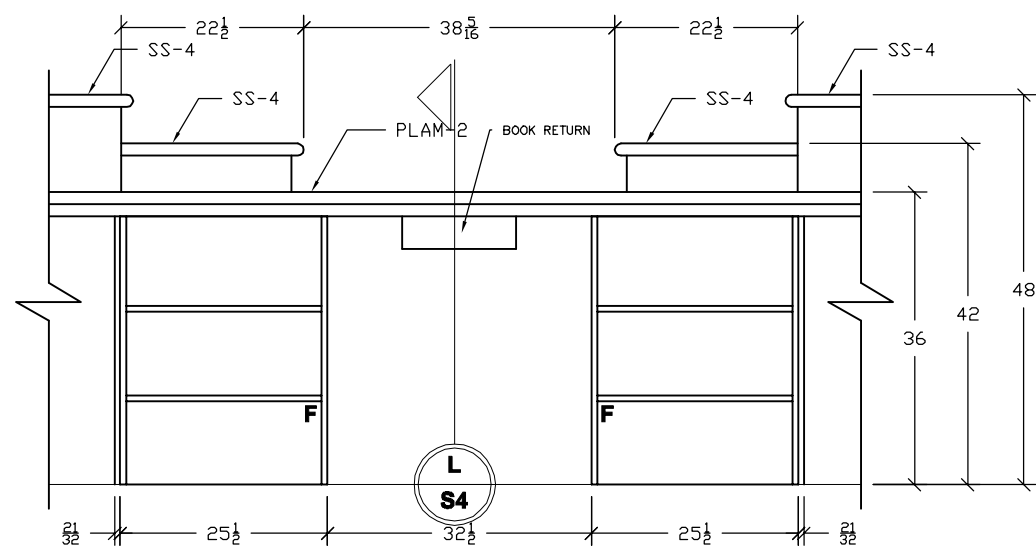
4 5 CIRCULATION DESK 102 ARCHITECTURAL REF: 4/A4-002 SCALE: 1/2" = 1'
