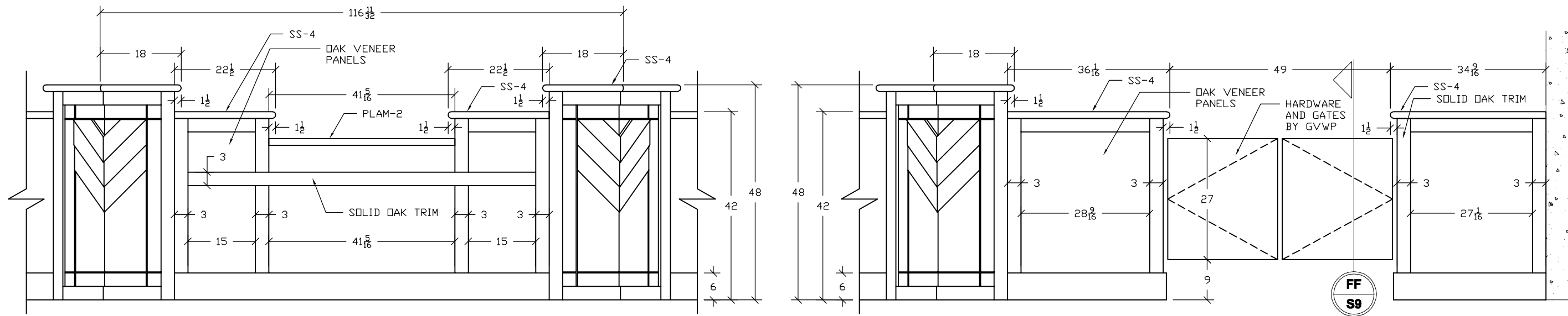
9 7 CIRCULATION DESK 102 ARCHITECTURAL REF: 9/A4-002 SCALE: 1/2" = 1'
