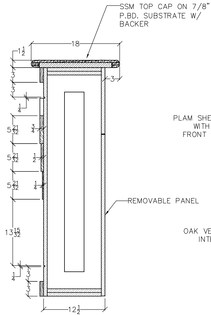
TYPICAL DESK CORNER SCALE: 1" = 1'
