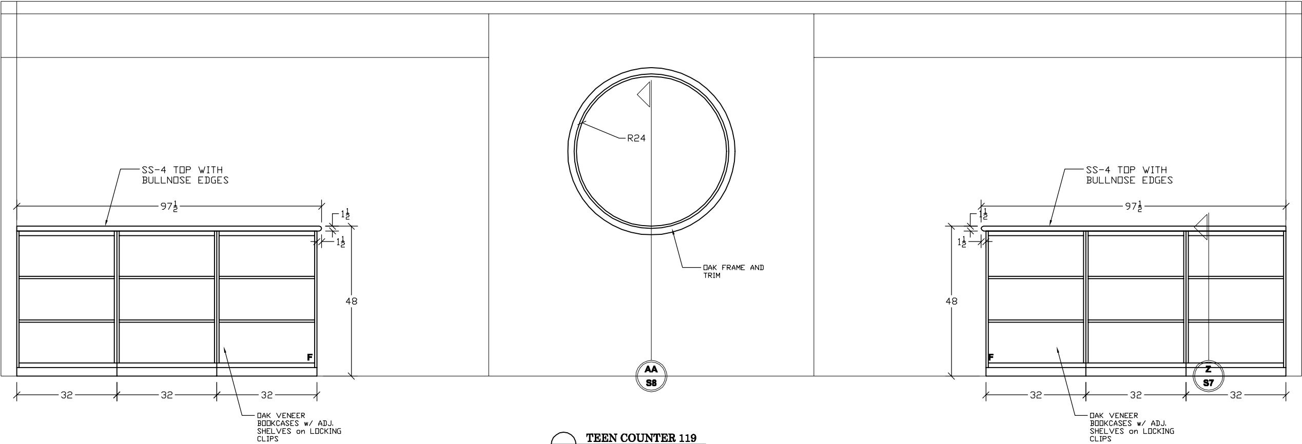
TEEN COUNTER 119 ARCHITECTURAL REF: 2/A4-005 SCALE: 3/8" = 1'
