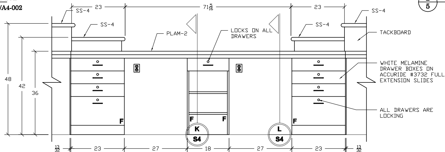
3 5 CIRCULATION DESK 102 ARCHITECTURAL REF: 3/A4-002 SCALE: 1/2" = 1'
