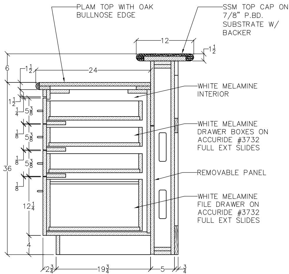
REFERENCE DESK SCALE: 1" = 1'
