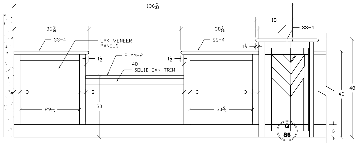
6 CIRCULATION DESK 102 6 ARCHITECTURAL REF: 6/A4-002 SCALE: 1/2" = 1'
