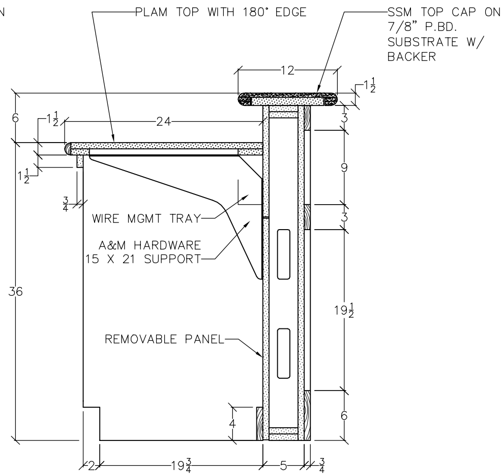
REFERENCE DESK SCALE: 1" = 1'
