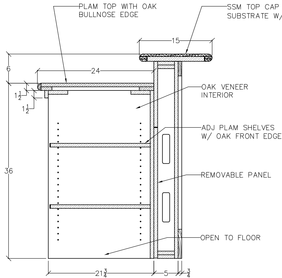
H CIRCULATION DESK SCALE: 1" = 1'
