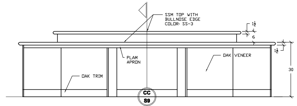
27 19 YOUTH COMPUTER DESK ARCHITECTURAL REF: 5/A4-006 SCALE: 3/8" = 1'
