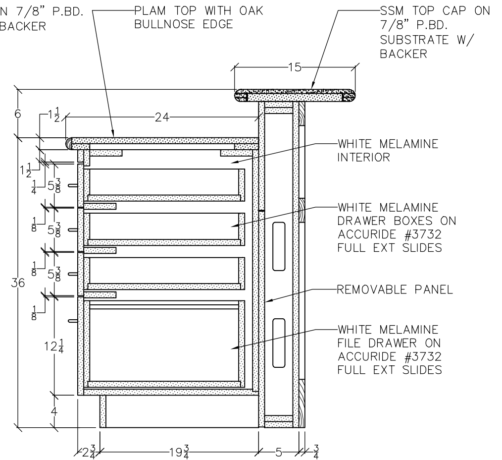
J CIRCULATION DESK SCALE: 1" = 1'
