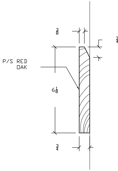
TYPICAL PICTURE RAIL SCALE: 3" = 1' GVWP TO PROVIDE 1,100 FT
