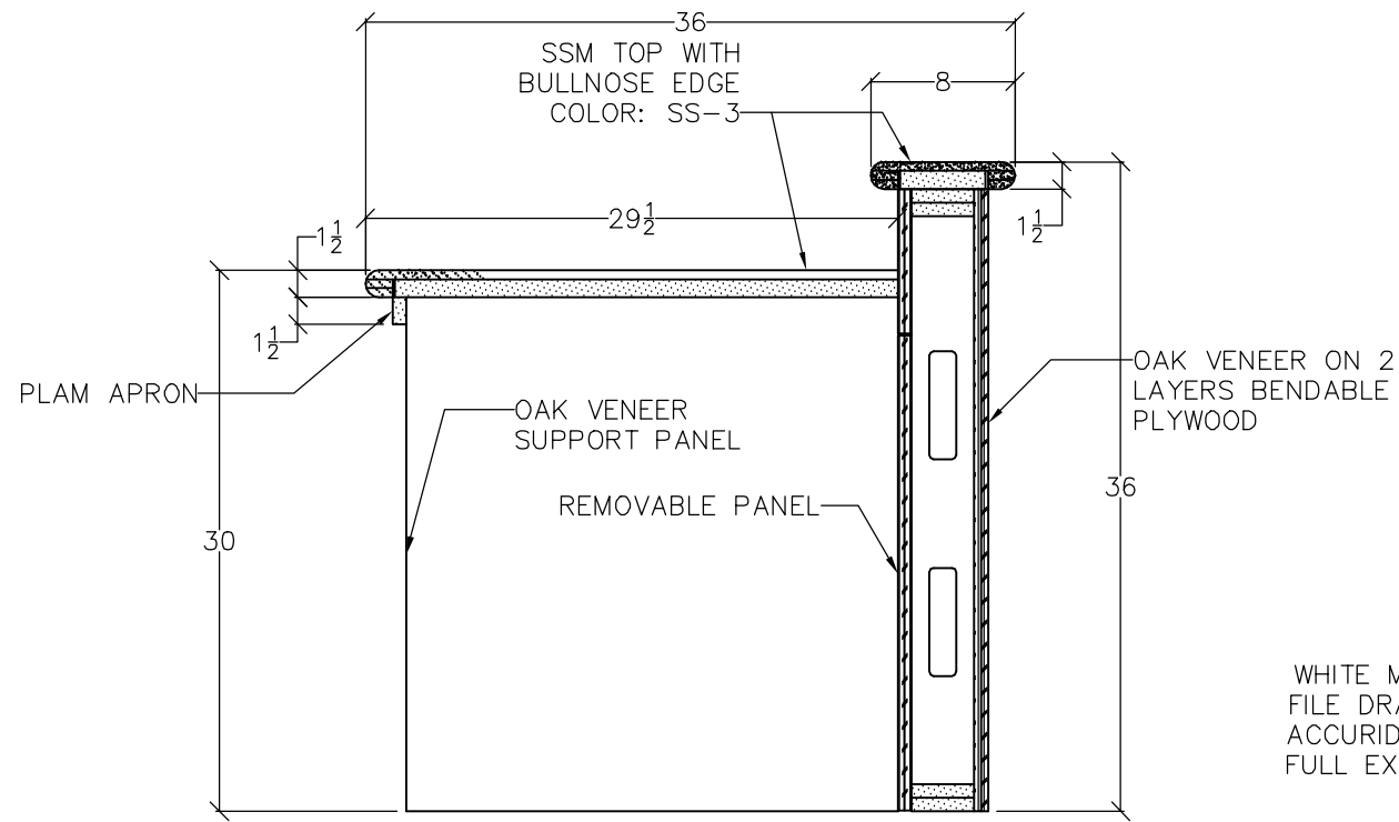
CC YOUTH COMPUTER DESK SCALE: 1" = 1'
