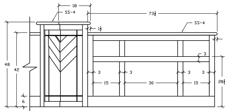
23 10 REFERENCE DESK 101 ARCHITECTURAL REF: 4/A4-002 SCALE: 3/8" = 1'
