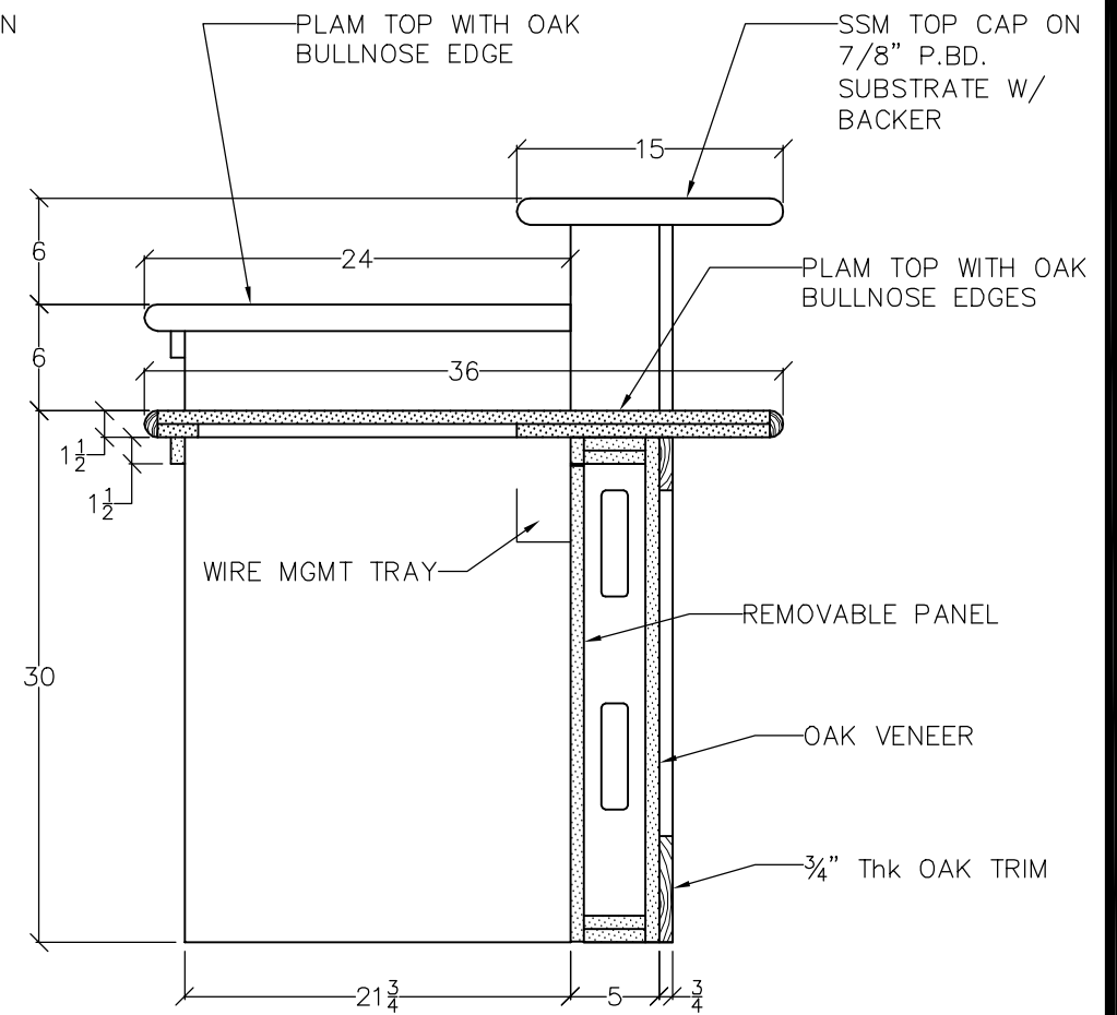
M CIRCULATION DESK SCALE: 1" = 1'
