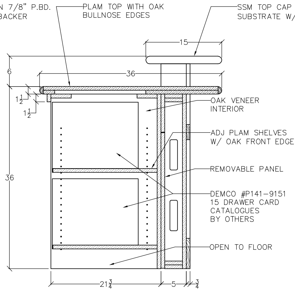
I CIRCULATION DESK SCALE: 1" = 1'
