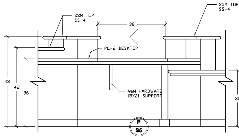
15 9 REFERENCE DESK 101 ARCHITECTURAL REF: 4/A4-002 SCALE: 3/8" = 1'
