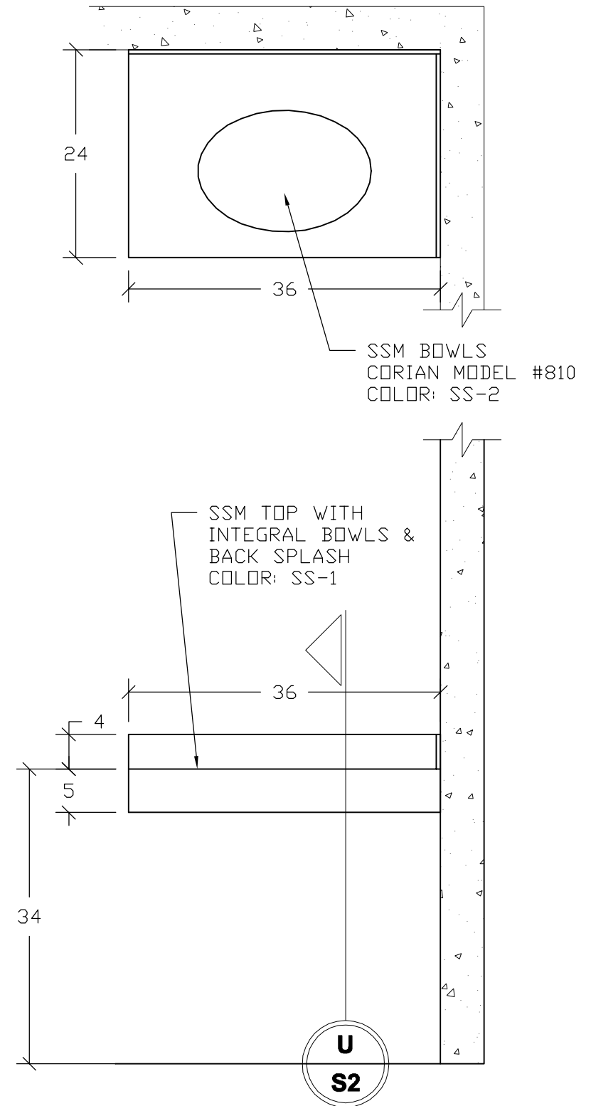
RESTROOM 107 ARCHITECTURAL REF: 3/A4-001 SCALE: 3/4" = 1'
