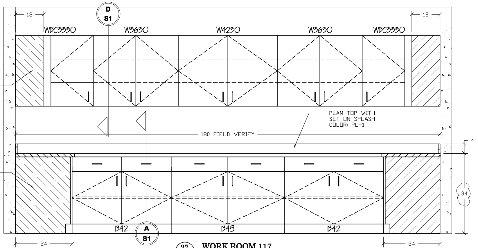
27 15A WORK ROOM 117 ARCHITECTURAL REF: 2/A4-005 SCALE: 1/2" = 1'
