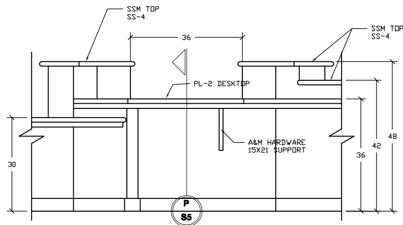
17 9 REFERENCE DESK 101 ARCHITECTURAL REF: 4/A4-002 SCALE: 3/8" = 1'
