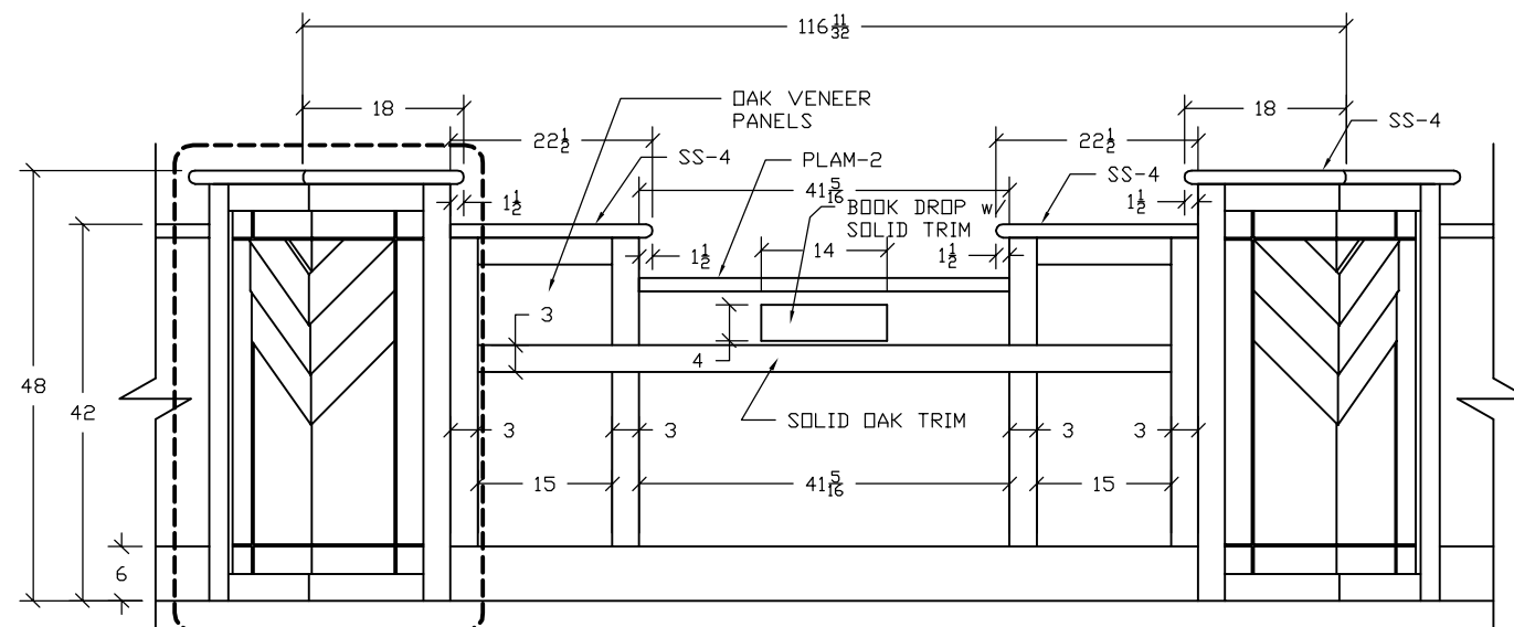
7 CIRCULATION DESK 102 6 ARCHITECTURAL REF: 7/A4-002 SCALE: 1/2" = 1'
